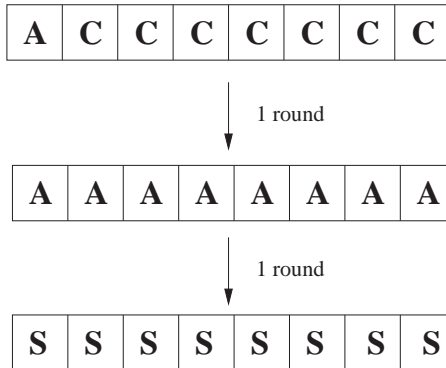
Fig. 1. The straightforward integral attack
