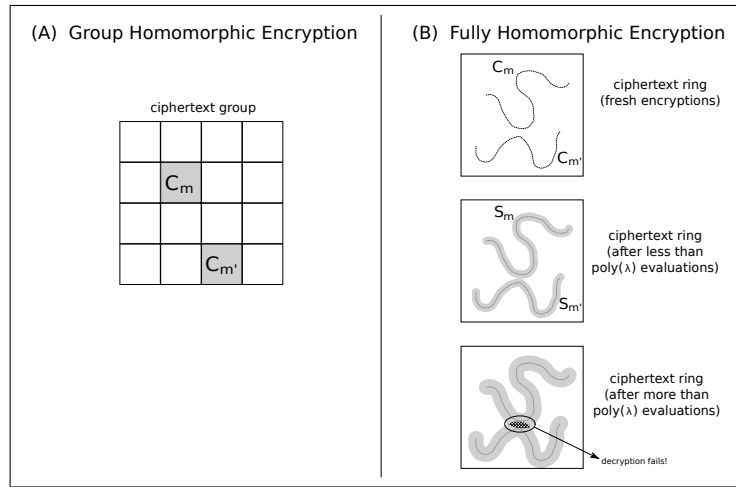
Fig. 1. Differences between group homomorphic encryption and FHE: (A) shows that each \mathcal{C}_m is a coset of \mathcal{C}_1 in \mathcal{C} (Fact 1), while the decryption is a group homomorphism; (B) shows first that \mathcal{C}_m and \mathcal{C}_{m'} are subsets and not necessarily cosets in \mathcal{C} , second that the decryption runs correctly on \text{poly}(\lambda) evaluations of ciphertexts, and third that the decryption might fail if exponentially many evaluations have been performed, meaning that the decryption is not necessarily group homomorphic.
