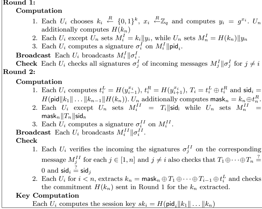
Fig. 4. GKE protocol of Bohli et al. [5]
