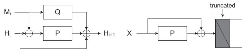
Fig. 2. Compression function and output transformation of Grøst1
