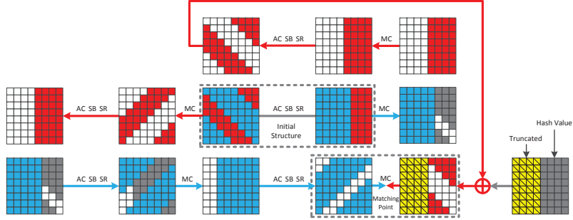
Fig. 4. Chunk separation of preimage attack on Grøstl-256's output transformation
