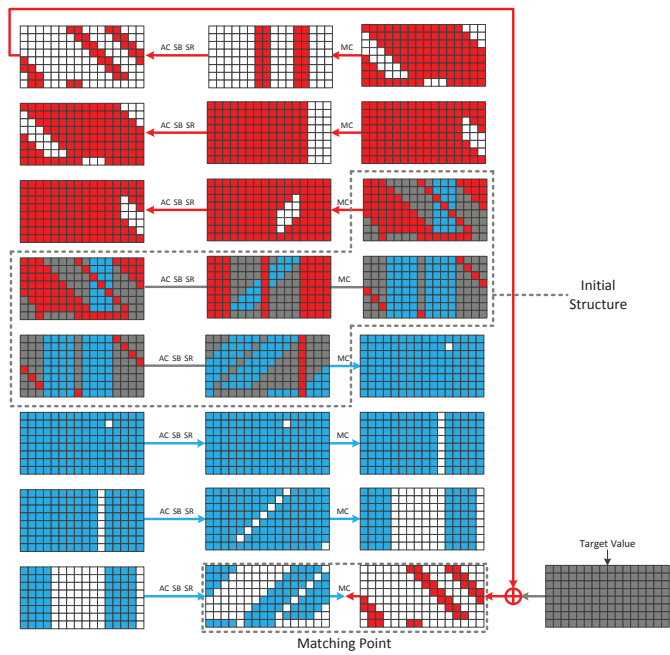
Fig. 10. Chunk separation of chosen position partial preimage attack on P(H') \oplus H' for Grøstl-512
