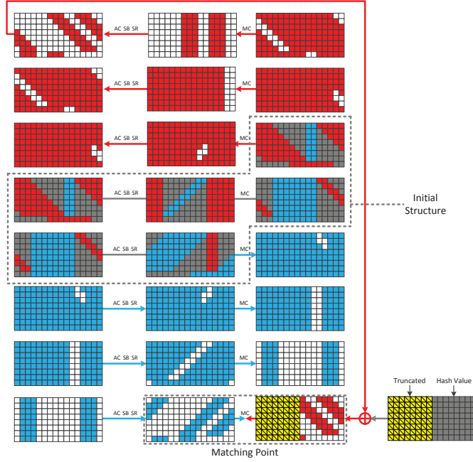
Fig. 9. Chunk separation of preimage attack on Grøstl-512's output transformation
