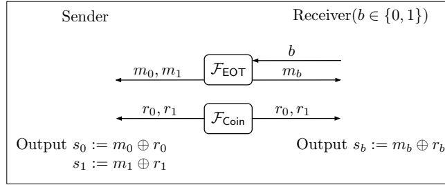
Fig. 10. UOT Protocol \Pi_{\text{UOT}} in the \{\mathcal{F}_{\text{EOT}}, \mathcal{F}_{\text{Coin}}, \mathcal{F}_{\text{Auth}}\} -Hybrid World from [35]
