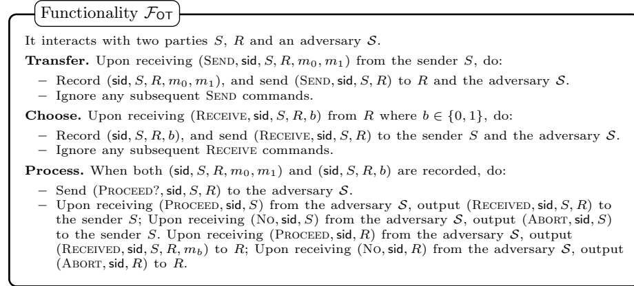
Fig. 3. The Ideal Functionality \mathcal{F}_{\text{OT}} for Oblivious Transfer
