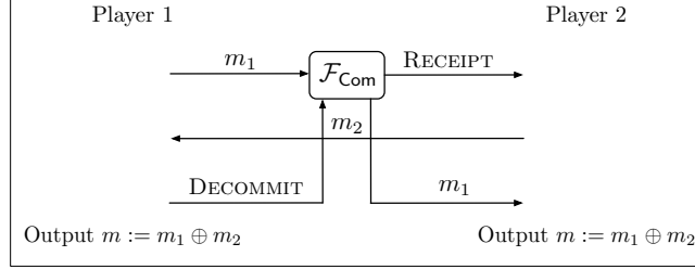
Fig. 11. Coin-Tossing Protocol \Pi_{\text{Coin}} in the \{\mathcal{F}_{\text{Com}}, \mathcal{F}_{\text{Auth}}\} -Hybrid World
