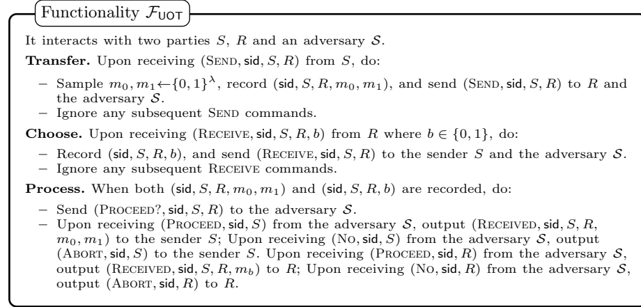
Fig. 4. The Ideal Functionality \mathcal{F}_{\text{UOT}} for Uniform Oblivious Transfer
