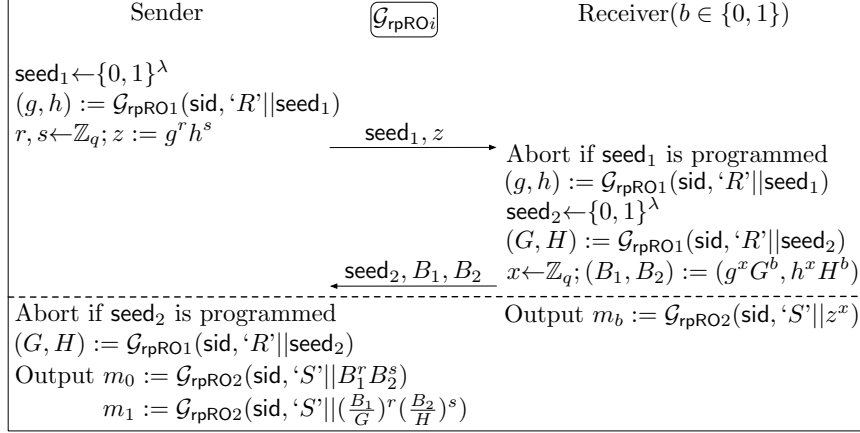
Fig. 14. 2-round EOT protocol \Pi_{\text{EOT-GrpRO}} in the \{\mathcal{G}_{\text{rpRO}}, \mathcal{F}_{\text{Auth}}\} -hybrid world, where \mathcal{G}_{\text{rpRO}} = \{\mathcal{G}_{\text{rpRO}1}, \mathcal{G}_{\text{rpRO}2}\} . Let \mathcal{G}_{\text{rpRO}1} : \{0, 1\}^* \rightarrow \mathbb{G} \times \mathbb{G} and \mathcal{G}_{\text{rpRO}2} : \{0, 1\}^* \rightarrow \{0, 1\}^\lambda .
