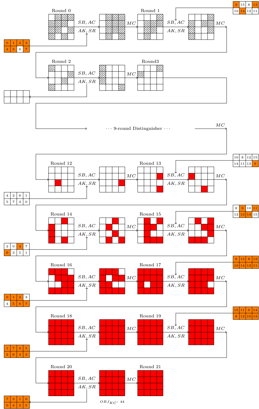
Fig. 33. 21-round Attack on SKINNY-64-192
