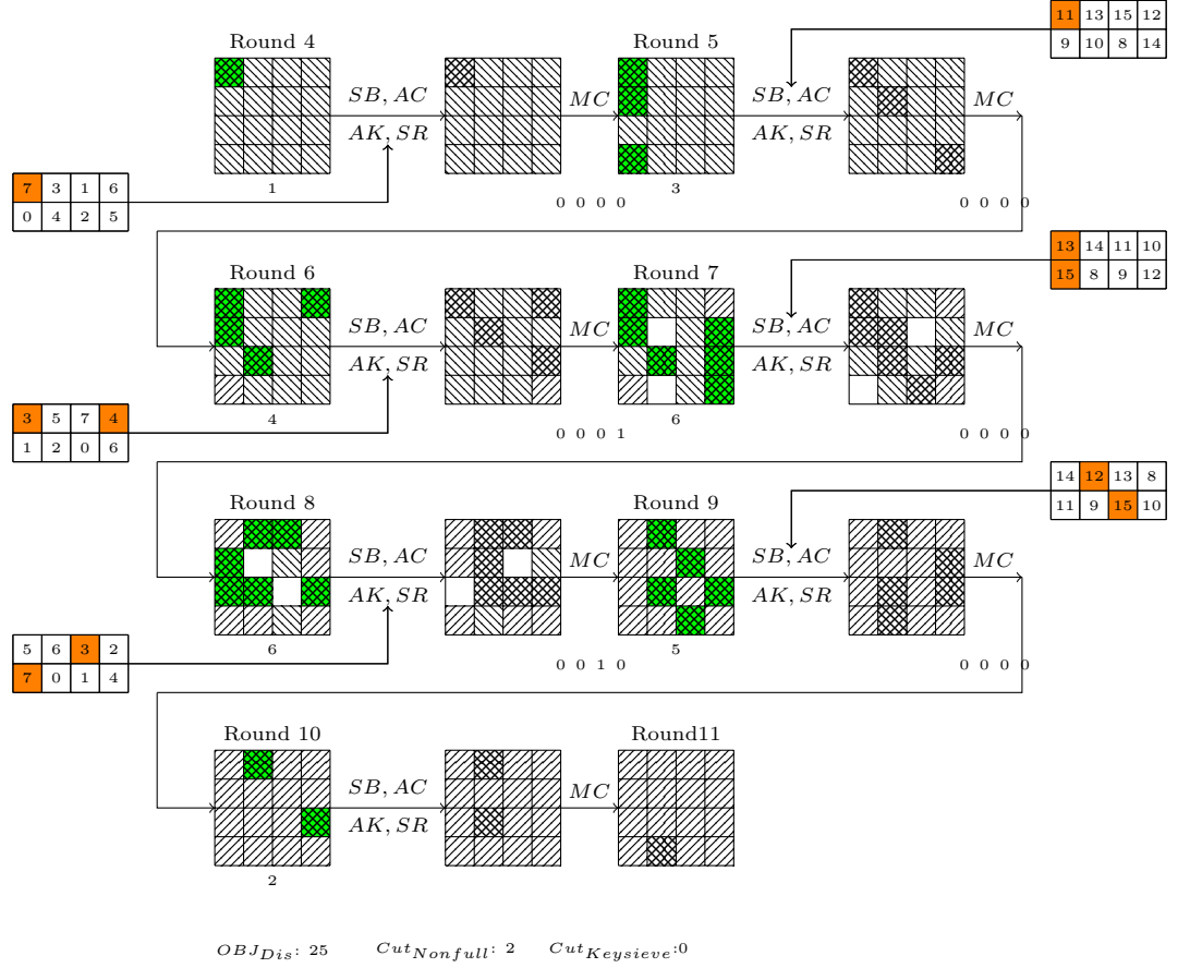
Fig. 28. 7-round Distinguisher of SKINNY-128-256
