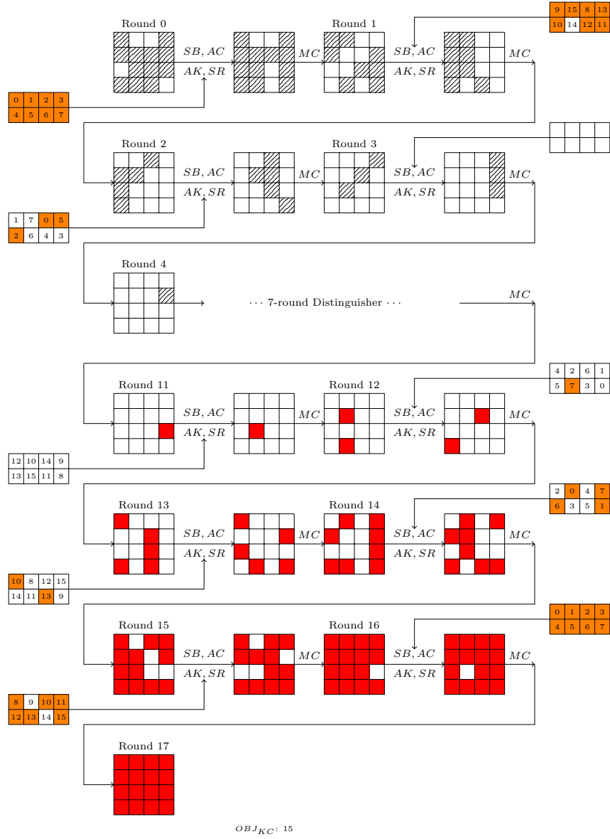
Fig. 35. 17-round Attack on SKINNY-128-128
