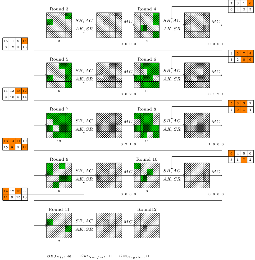
Fig. 32. 9-round Distinguisher of SKINNY-64-192
