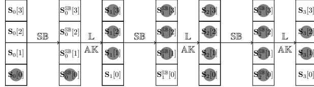
Fig. 7. A truncated differential trail on the toy cipher
