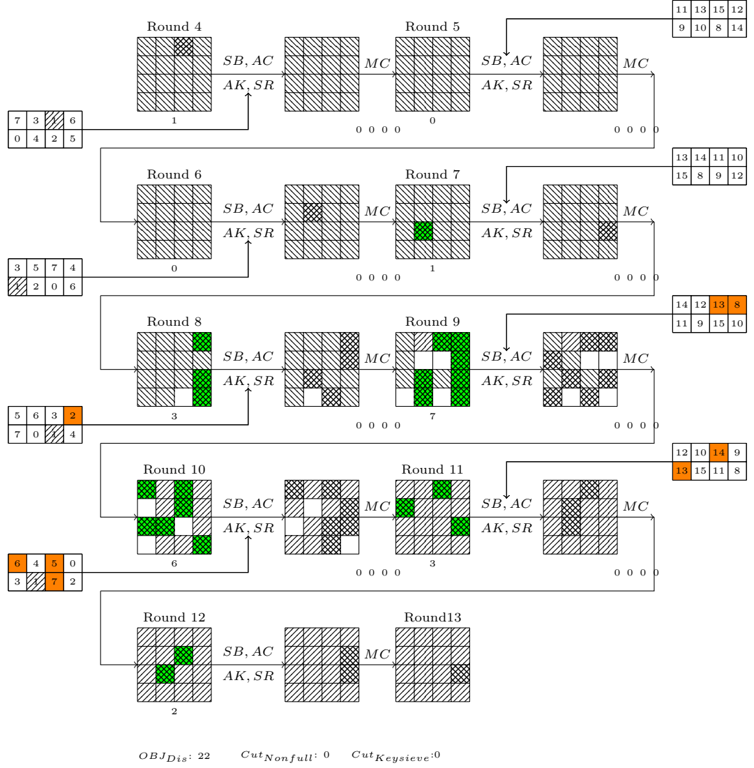
Fig. 12. 9-round Distinguisher of SKINNY-128-256
