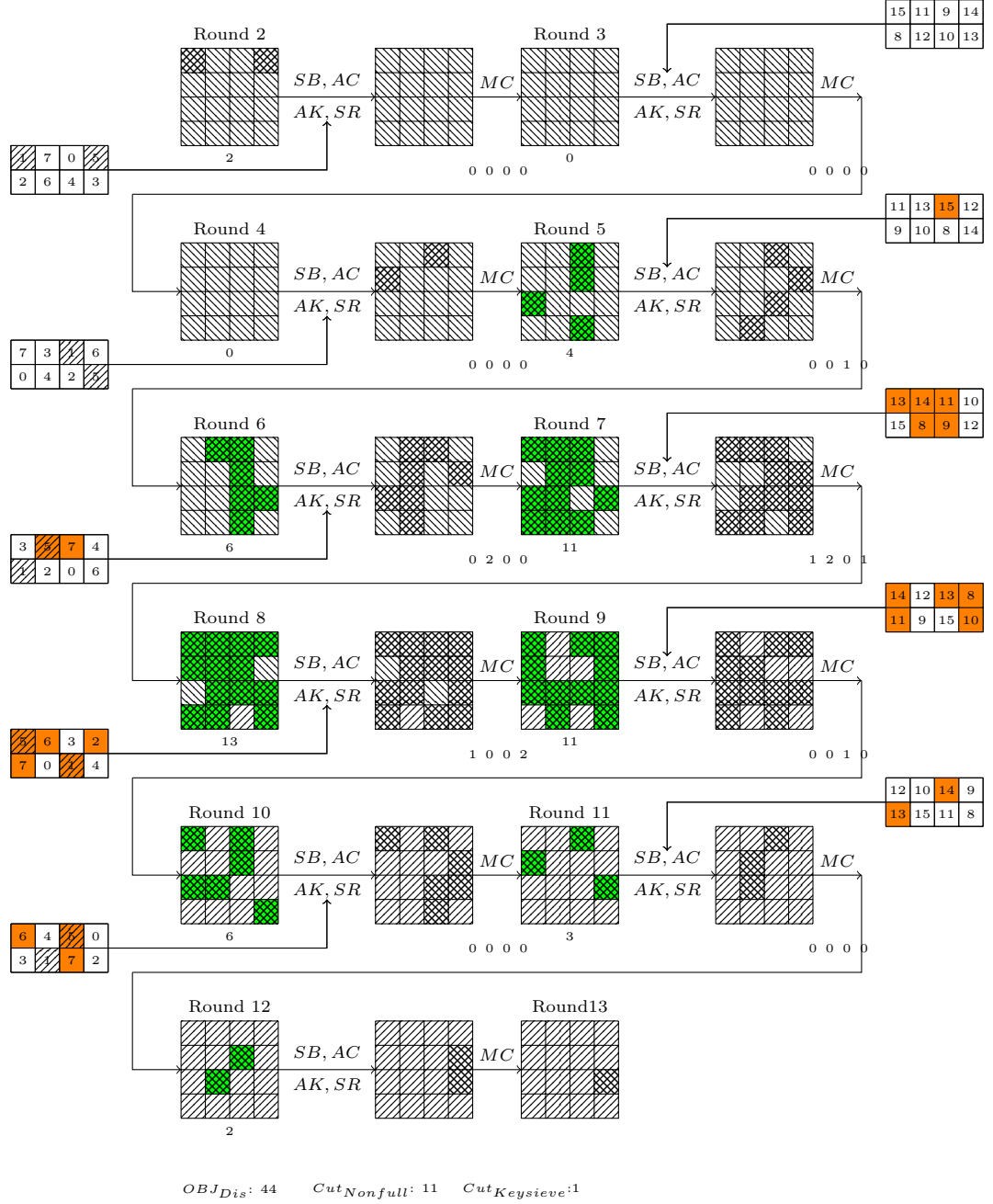
Fig. 22. 11-round Distinguisher of SKINNY-64-192
