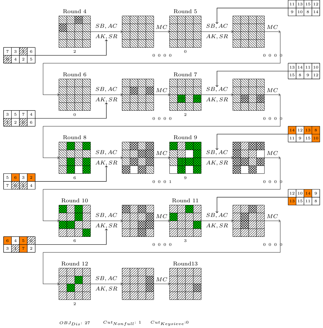
Fig. 18. 9-round Distinguisher of SKINNY-64-128
