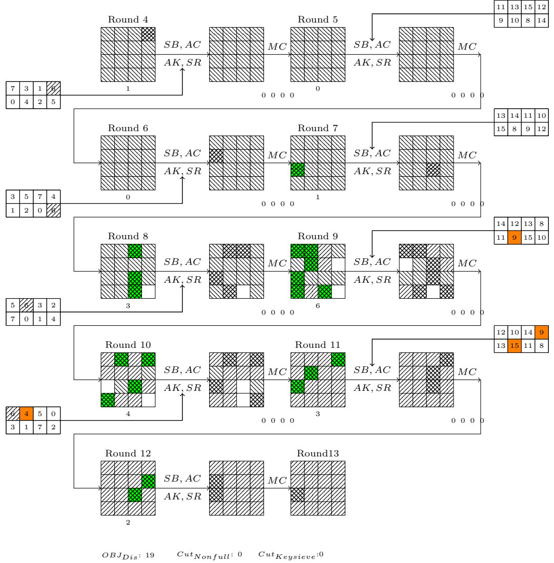
Fig. 14. 9-round Distinguisher of SKINNY-128-256
