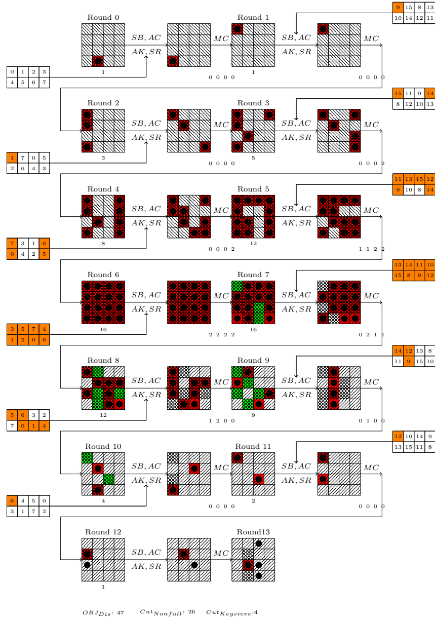
Fig. 42. 13-round Distinguisher on SKINNY-128-384
