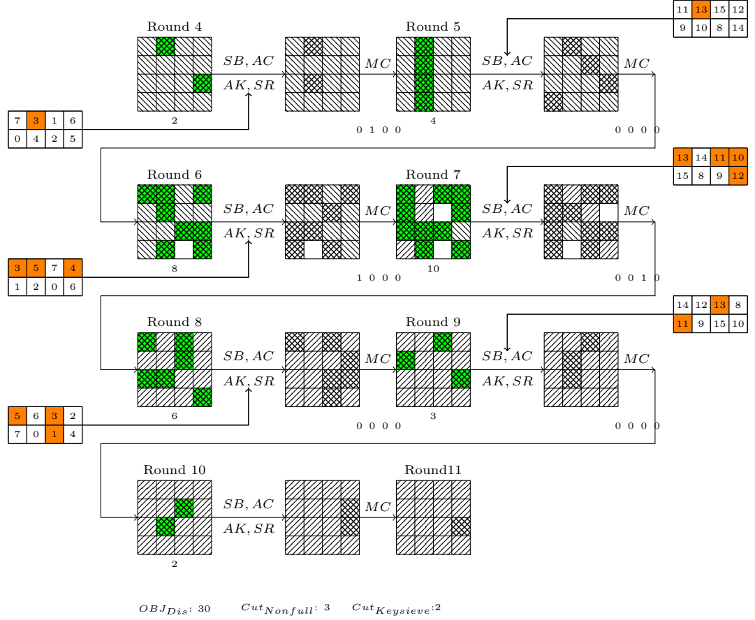
Fig. 38. 7-round Distinguisher of SKINNY-64-128
