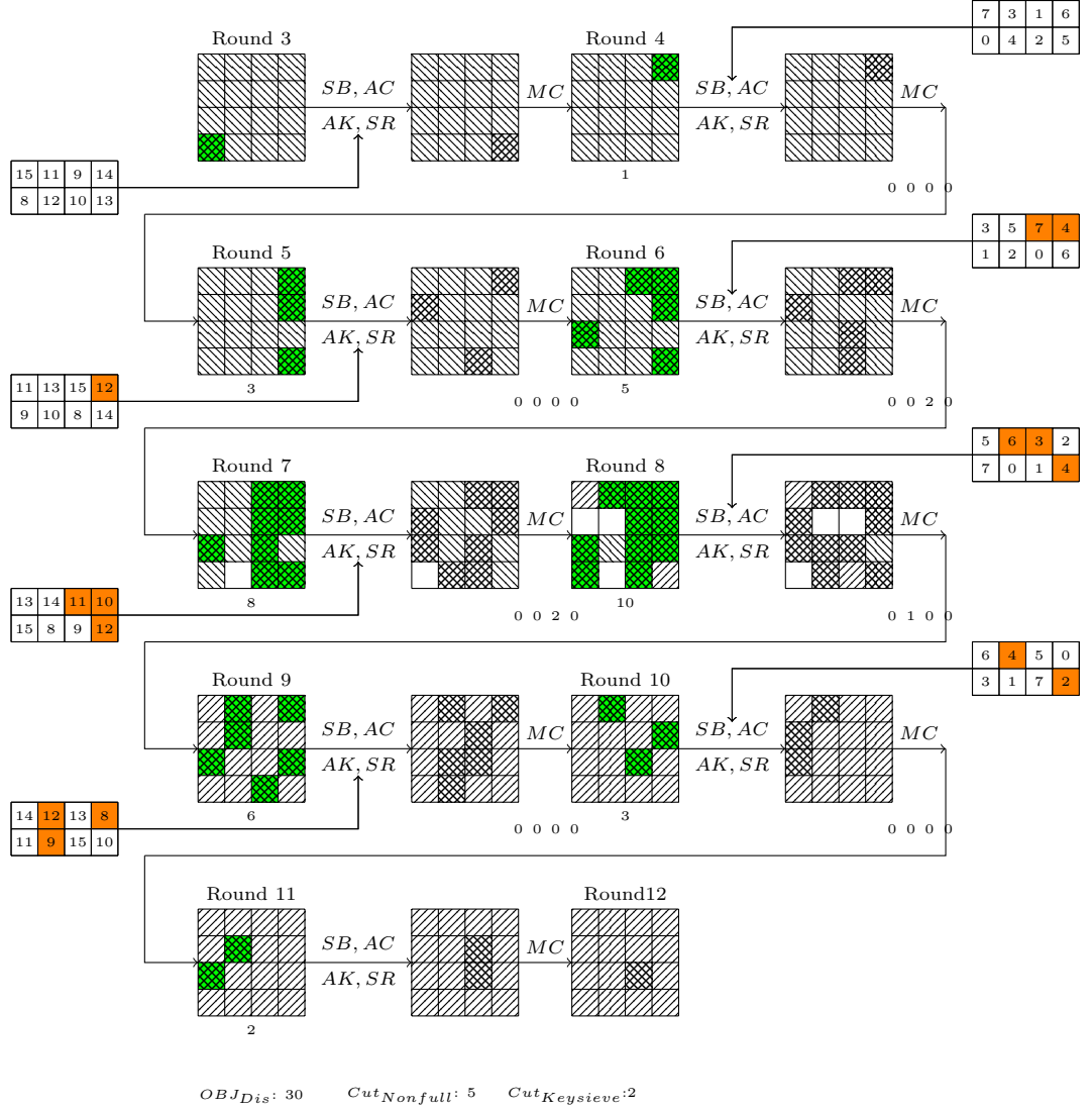
Fig. 26. 9-round Distinguisher of SKINNY-128-256
