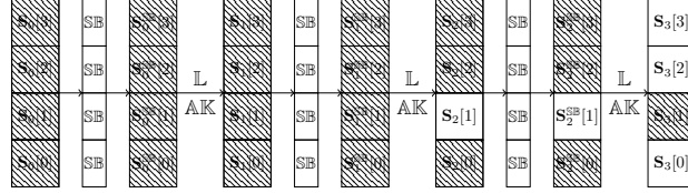
Fig. 5. A valid backward determination on toy cipher
