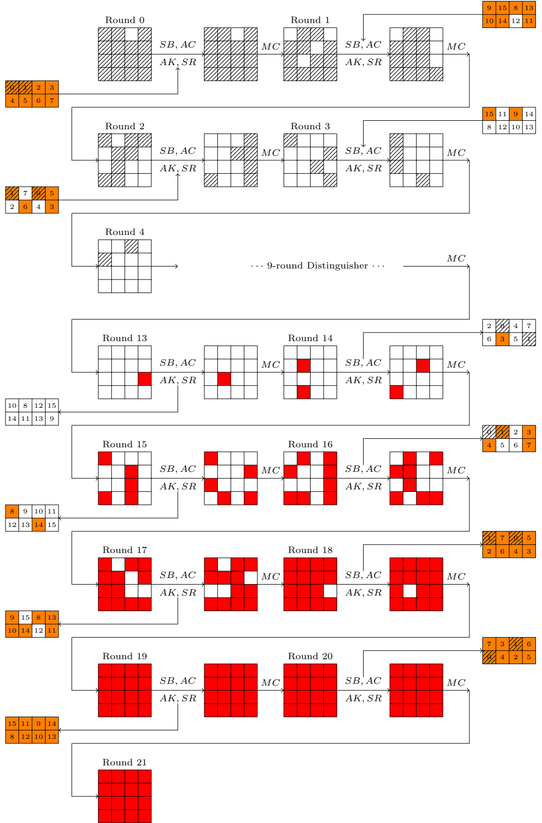
Fig. 19. 21-round Attack on SKINNY-64-128
