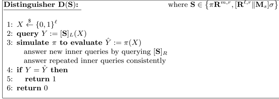
Fig. 2: The distinguisher \mathbf{D} for the proof of Theorem 2.
