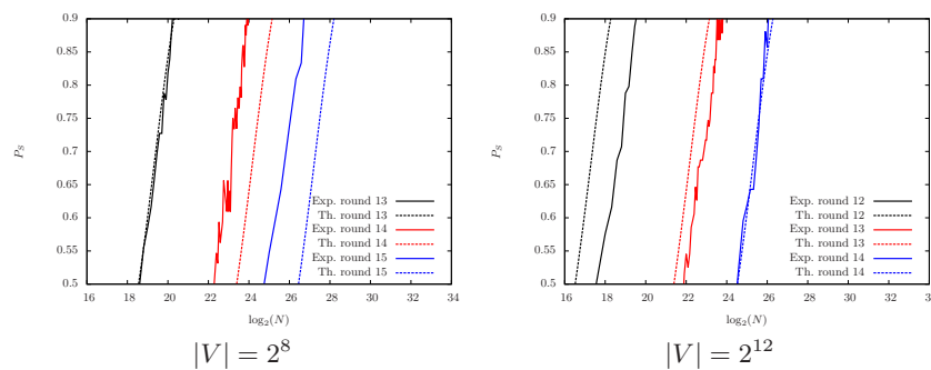
Fig. 2. Data complexity of attacks on 12, 13, 14 rounds of PUFFIN
