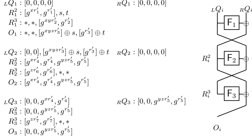
Fig. 2. An adaptive three query distinguishing attack for L\psi_{2n}[F_1F_2F_3] .
