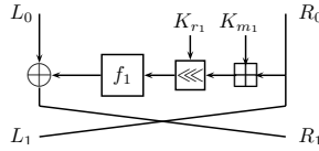
Fig. 4. The First Round of CAST-128
