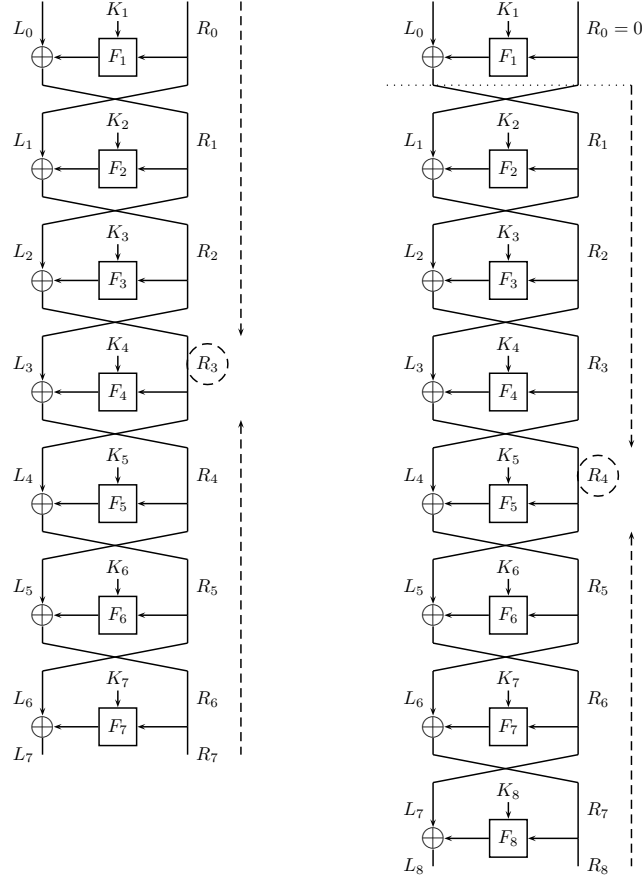
Fig. 2. On the Left: 7-Round MITM Attack. On the Right: 8-Round Splice-and-Cut Attack.
