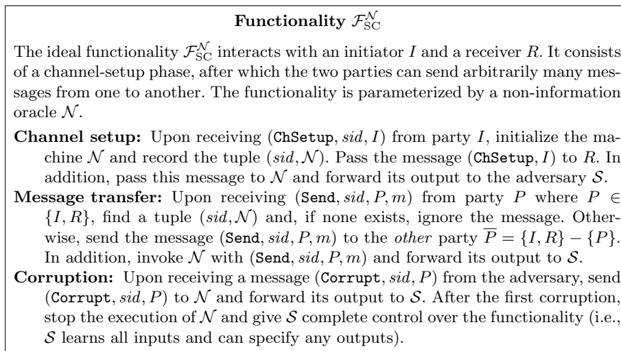
Fig. 1. The parameterized secure-channel ideal functionality, \mathcal{F}_{\text{SC}}^{\mathcal{N}} .
