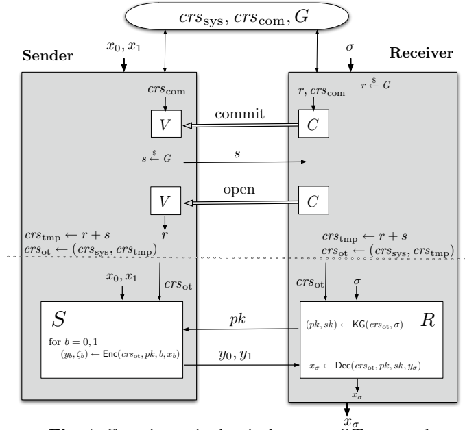
Fig. 4. Generic semi-adaptively secure OT protocol.
