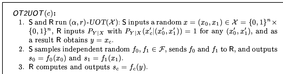
Fig. 2. Protocol OT2UOT for Rand1-2 OT \ell .
