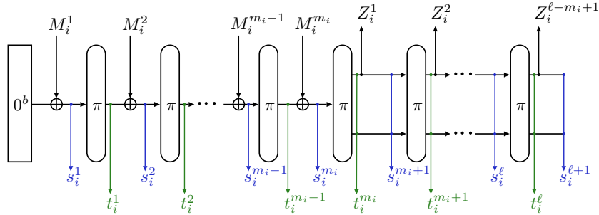
Fig. 3: Processing the i^{\text{th}} query.
