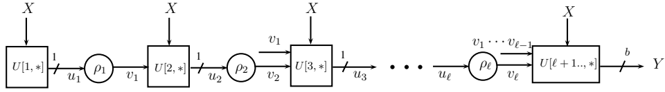
Fig. 1: Linear Mode: Here U[i, *] means the i^{\text{th}} block row which maps (X, v_1, \dots, v_{i-1}, 0^{\ell-i+1}) to u_i . Finally, U[l+1.. ; *] maps the input X and intermediate output vector v to the output Y consisting of b blocks.
