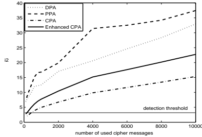
Fig. 5. Second attack-efficient index
