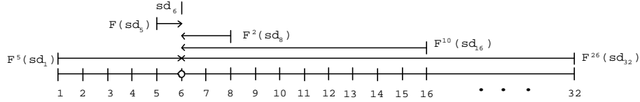
Fig. 3. Key assignment to u_6 in B1
