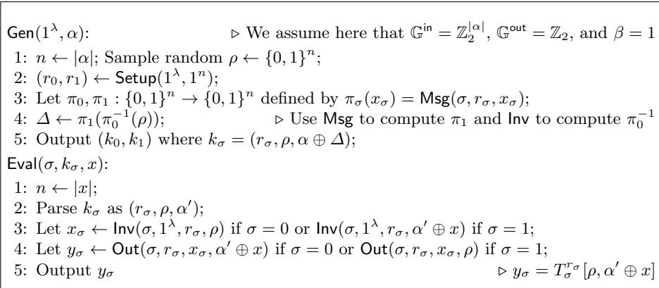
Fig. 1: DPF from online-optimal shared equality protocol ( Setup , Msg , Out , Inv ).
