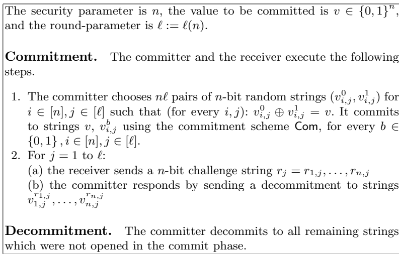
Fig. 1. The PRS Preamble based on \text{Com} .
