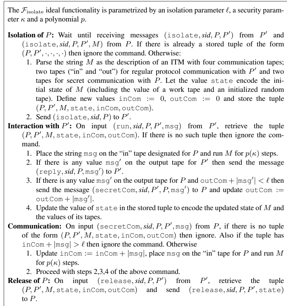
Fig. 1. The \mathcal{F}_{\text{isolate}} Ideal Functionality
