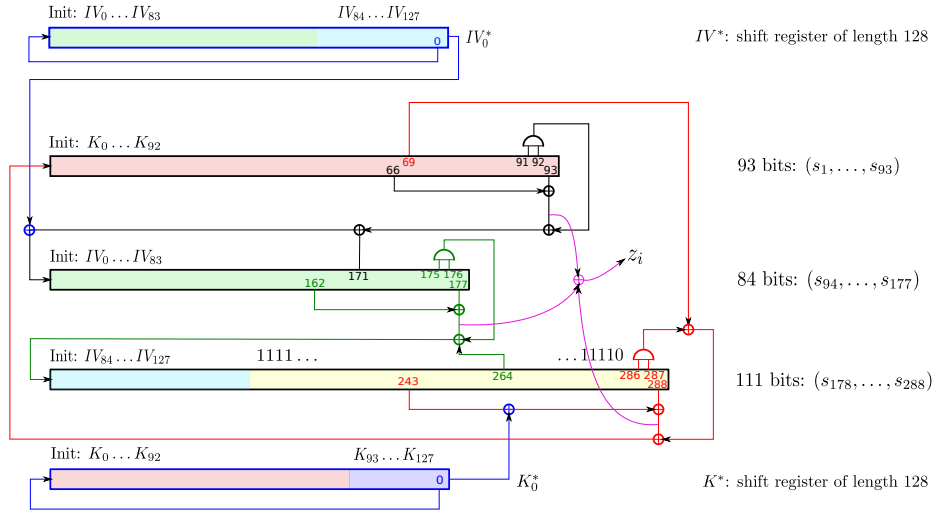
Fig. 2. Kreyvium. The three registers in the middle correspond to Trivium. The modifications defining Kreyvium correspond to the two registers at the top and at the bottom.
