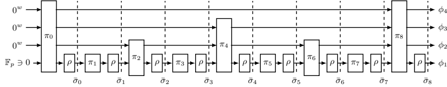
Fig. 3: Illustration of the computation of \bar{\sigma}_\Pi = (\bar{\sigma}_0, \dots, \bar{\sigma}_N) with n = 3, N = 2^n = 8 .
