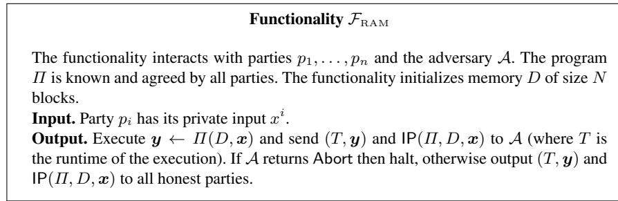
Fig. 1. Ideal execution of \Pi(N, \mathbf{x}) with abort.
