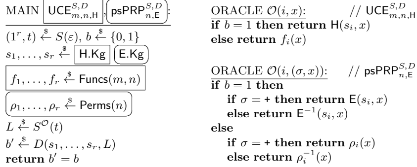
Fig. 1: Games to define UCE and psPRP security. Here, S is the source and D is the distinguisher. Boxed statements are only executed in the corresponding game.
