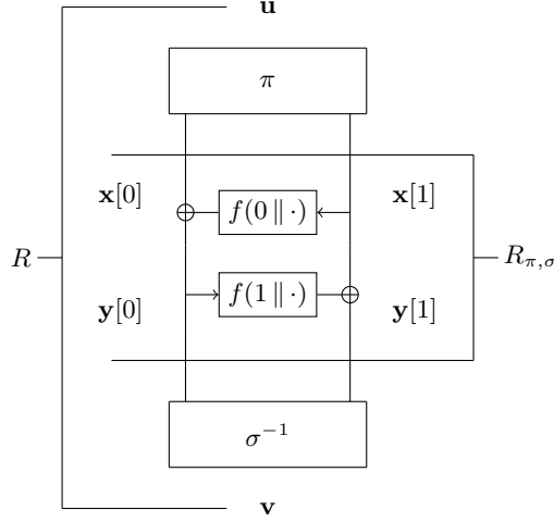
Fig. 6: The NR construction instantiated with a permutation family \mathsf{P} on 2n -bits such that \mathsf{P}^{-1} is (\varepsilon, k \cdot t) -wise independent where \pi = \mathsf{P}(s^{\text{in}}, \cdot) and \sigma = \theta(\mathsf{P}(s^{\text{out}}, \cdot)) for s^{\text{in}}, s^{\text{out}} \leftarrow \mathsf{P.Kg} . Here, \theta is a permutation on 2n -bits such that for all \mathbf{x} \in \{0, 1\}^{2n} we have \theta(\mathbf{x} = x_0 \| x_1) = x_1 \| x_0 . For some k -ary strongly-evasive relation R , we construct a 2-Feistel evasive relation R_{\pi, \sigma} by transforming every (\mathbf{u}, \mathbf{v}) \in S where S \in R , by applying \pi to \mathbf{u} and \sigma to \mathbf{v} .
