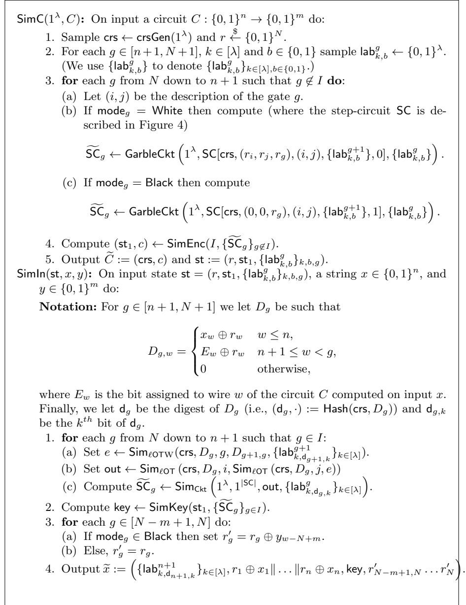
Figure 5: Garbling in configuration \text{conf} = (I, \{(h, \text{mode}_h)\}_{h \in [n+1, N]}) .
