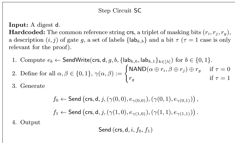
Figure 4: Description of the Step Circuit
