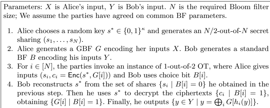
Fig. 3. The malicious-secure protocol of DCW [8] .
