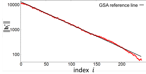
Fig. 2. Semi-log graph of \|\mathbf{b}_i^*\| of a 240-dimensional highly reduced basis
