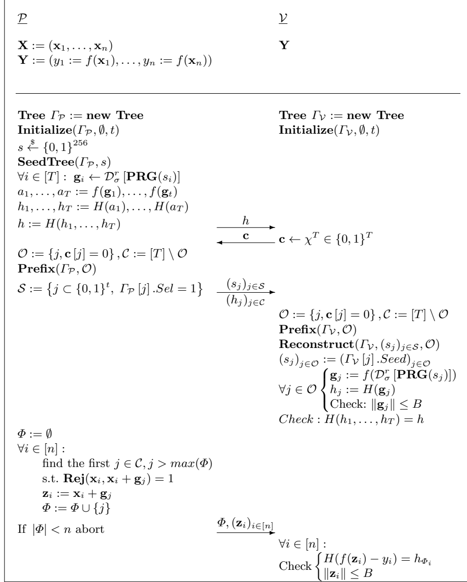
Fig. 4. Our first construction: For \alpha \geq 2 , we fix T = 5\alpha n and \chi the bernoulli distribution of parameter 1/\alpha . We obtain an imperfect proof of knowledge with imperfection \frac{k}{\log \alpha} + 1 . The communication complexity only has a small dependence on \log \alpha .
