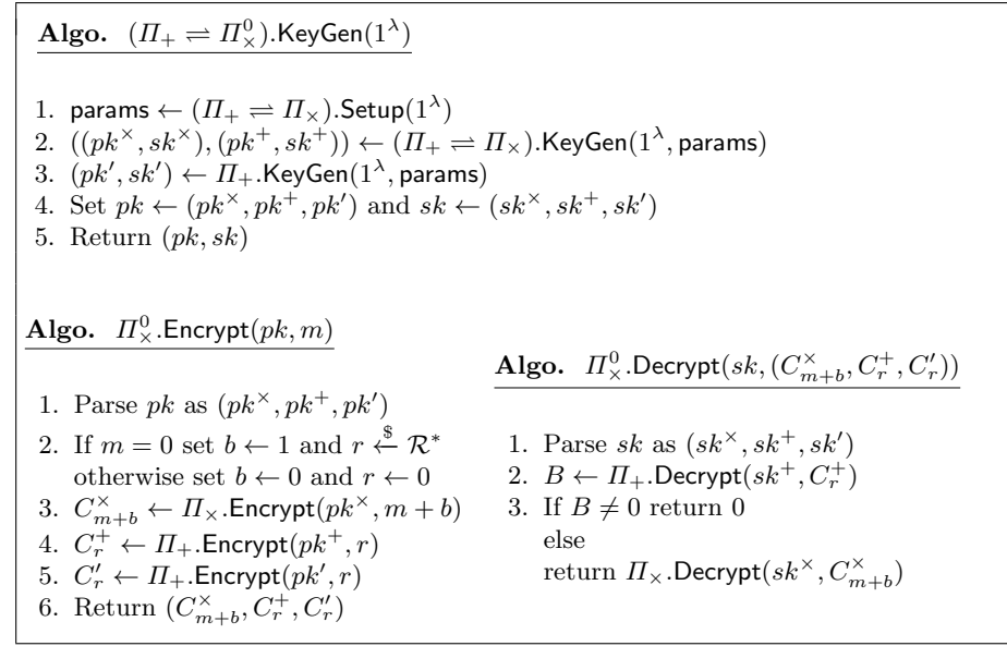
Fig. 4. \Pi_\times over \mathcal{R} : \Pi_\times^0
