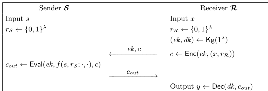
Figure 3. Oblivious Two-Party Protocol
