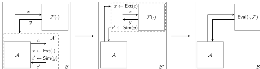
Figure 2. Oblivious reduction part 2 of 2.
