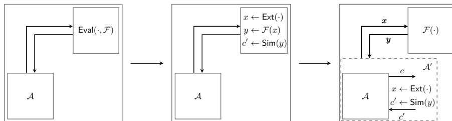
Figure 1. Oblivious reduction part 1 of 2.
