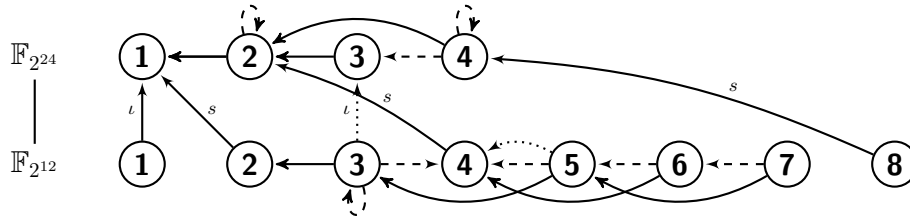
Fig. 1. This diagram depicts the set of strategies employed to eliminate elements over \mathbb{F}_{2^{12}} of degree up to 8. The encircled numbers represent the degrees of elements over \mathbb{F}_{2^{12}} on the bottom row, and over \mathbb{F}_{2^{24}} on the top row. The arrows indicate how an element of a given degree is rewritten as a product of elements of other degrees, possibly over the larger field. Unadorned solid arrows indicate the maximum degree of elements obtained on the l.h.s. of the Gröbner basis elimination method; likewise dashed arrows indicate the degrees of elements obtained on the r.h.s. of the Gröbner basis elimination method, when these are greater than those obtained on the l.h.s. Dotted arrows indicate a fall-back strategy when the initial strategy fails. An s indicates that the element is to be split over the larger field into two elements of half the degree. An l indicates that an element is promoted to the larger field. Finally, a loop indicates that one must use a recursive strategy in which further instances of the elimination in question must be solved in order to eliminate the element in question.
