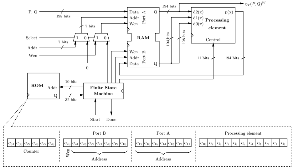
Fig. 2. Architecture of the \eta_T pairing accelerator.
