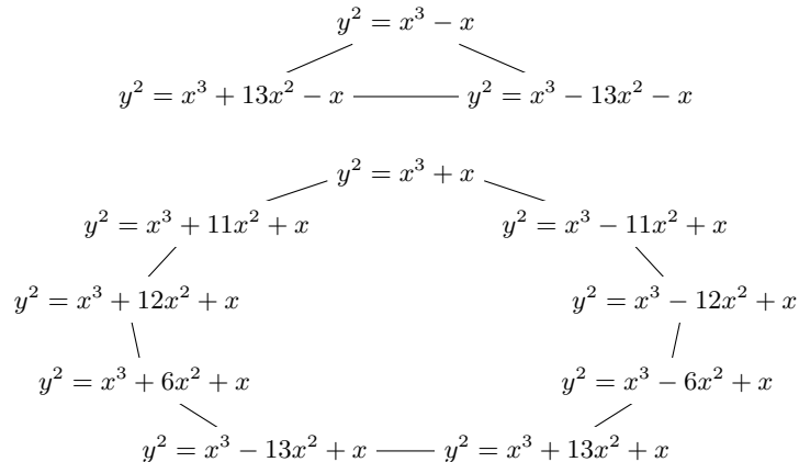
Figure 2. The two supersingular components of G_{\mathbb{F}_{83},3} . The curves in the top component have \mathbb{F}_p -rational endomorphism ring \mathbb{Z}[(1 + \sqrt{-83})/2] , while those in the lower component correspond to \mathbb{Z}[\sqrt{-83}] . Running clockwise through these components corresponds to the repeated action of [(3, \pi - 1)] .
