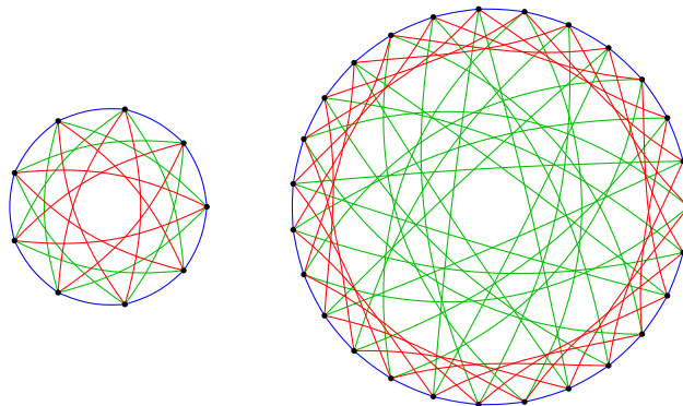
Figure 1. Union of the supersingular \ell -isogeny graphs for \ell \in \{3, 5, 7\} over \mathbb{F}_{419} . CSIDH makes use of the larger component, corresponding to curves whose ring of \mathbb{F}_{419} -rational endomorphisms is isomorphic to \mathbb{Z}[\sqrt{-419}] .
