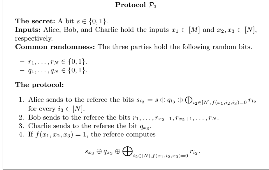
Fig. 1. A linear 3-party CDS protocol \mathcal{P}_3 for a 3-input function f : [M] \times [N] \times [N] \rightarrow \{0, 1\} .
