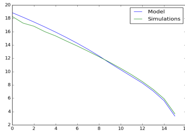
Fig. 3: Comparison between our model and our simulations for the number of elements in each pool at each step for p, w = 8, 16 , in log scale.
