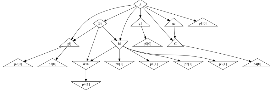
Fig. 4: Dependency graph for the ACF IB-KEM [2]. The master public key consists of g , gij , and g1 . Secret key derivation uses hi as the auxiliary information and skID as the secret key for identity ID . The pairing p0 and the ciphertext C are used in the encapsulation process, decapsulation uses the pairings p1 , p2 , and p3 , and the key is calculated from the encapsulation using p4 . In the reduction, Bi and gc are derived from the q -wBDHI assumption.
