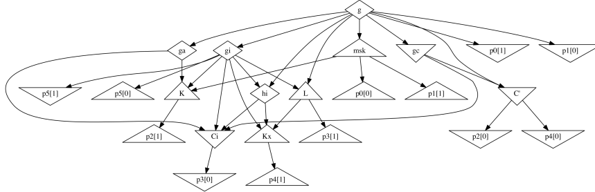
Fig. 5: Dependency graph for the Waters ABE scheme [42]. The public key consists of g , ga , and hi , and is computed using the pairing p0 . msk denotes the master secret key and the secret key consists of K , Kx , and L . Encryption uses the pairing p1 and produces C' and Ci , and decryption uses the pairings p2 , p3 , and p4 . In the reduction, gi and gc are derived from the q -BDHE assumption, and the pairing p5 is used to simulate the pairing p0 .
