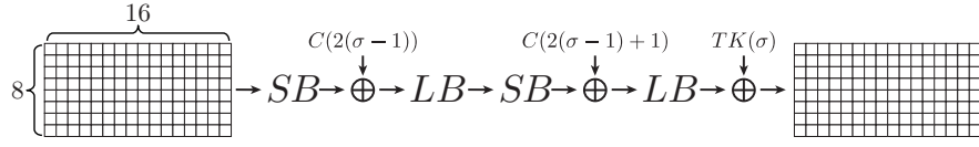
Fig. 3. The \sigma th step function of Scream
