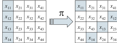
Fig. 3. ShiftRows transformation of Rijndael
