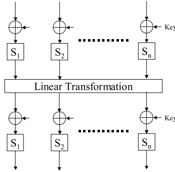
Fig. 2. 2 rounds of SPN structures
